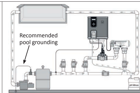
Installation on a by-pass
