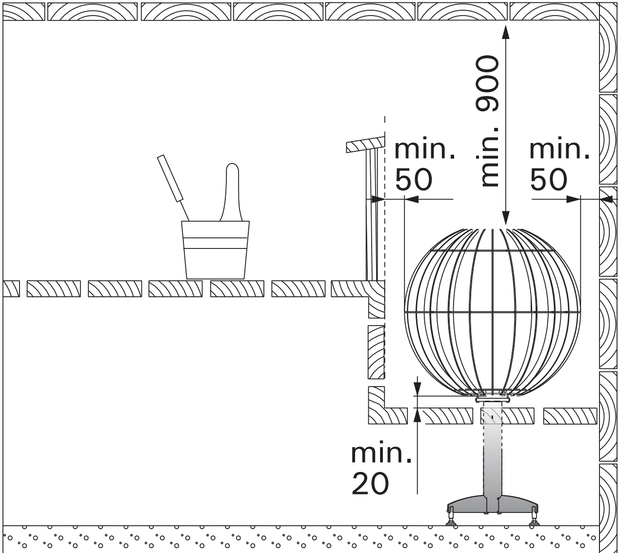
Safety distances (all dimensions in millimeters)
