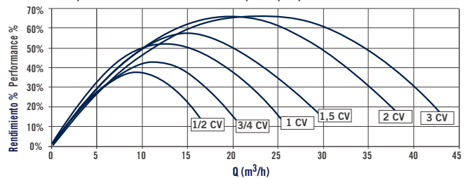
Curva rendimiento total-caudal bombas trifásicas Total performance-flow curve for three-phase pumps
