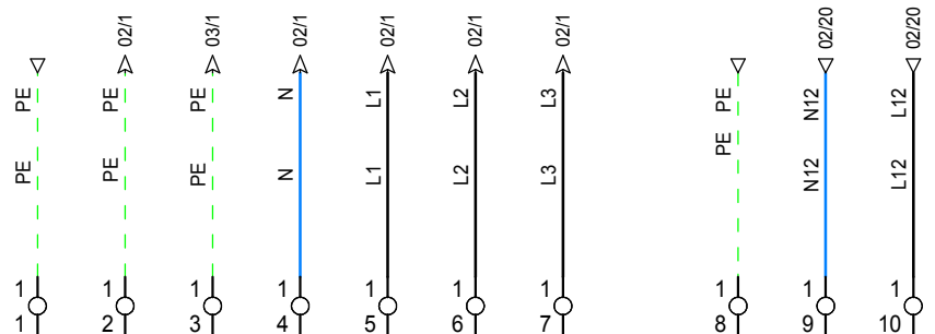
POWER SUPPLY 3PH + NEUTRAL
