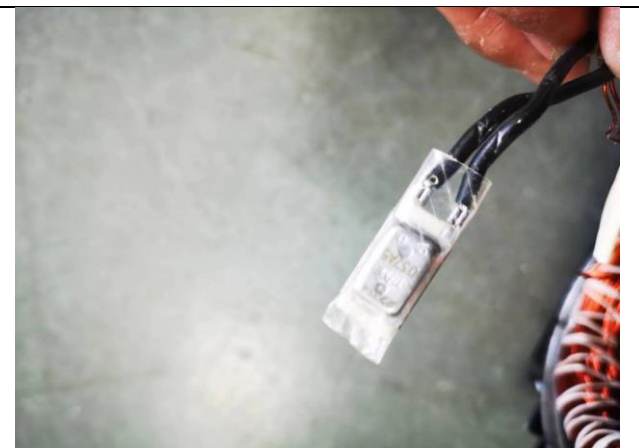
Photo 12 – Motor thermal protector of all models
