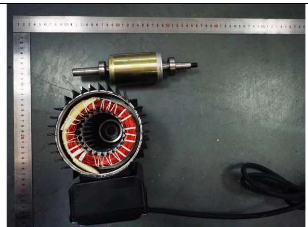
Photo 11 – Motor of model 04012G04
