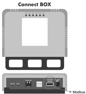
Connect Box Modbus Connector
