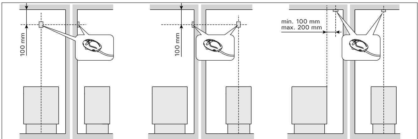
The place of the sensor of the control unit C150 in connection with floor-mounted heaters
