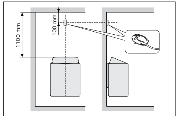
The place of the sensor in connection with wall-mounted heaters
