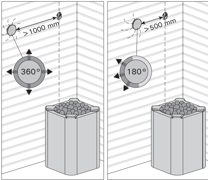
Sensor's minimum distance from an air vent
