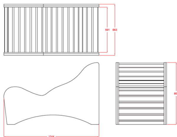
73901 (Infrared lamps)
