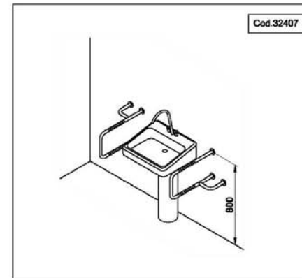
APOYO MURAL WALL SUPPORT APPUI MURAL
