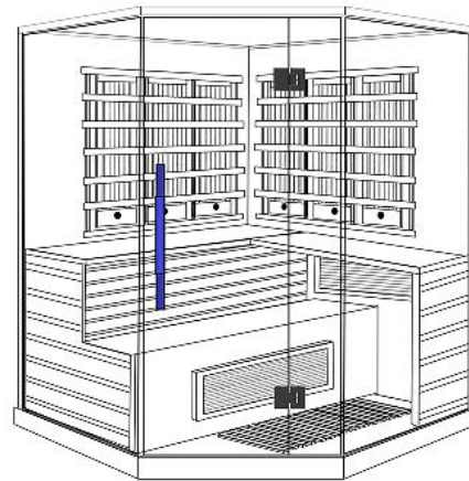
(14) Install Door handle and Glass seal
