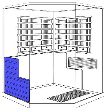
(7) Screw Left support panel to Left rear panel and Floor panel with Screw M3.5*40
