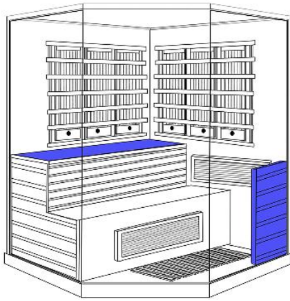
(11) Put Upper bench on Upper support panel, Install Right support panel to Right rear panel and Floor panel with Screw M3.5*40.
