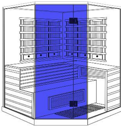
(13) Glass door and Small front window are pre-connected with Hinges, install them to Ceiling panel and floor panel with Deco screw set.
