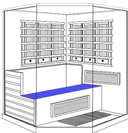
(9) Plug in the connector behind bench heater then put Lower bench onto Lower support panel:
