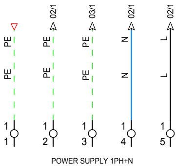
POWER SUPPLY 1PH+N
