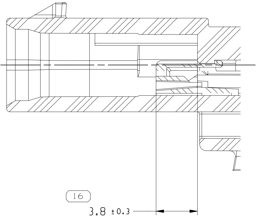
DELIVERY CONDITION TO WIRE ASSEMBLY PLANT PLR PRE-STAGED POSITION BEFORE TERMINALS
