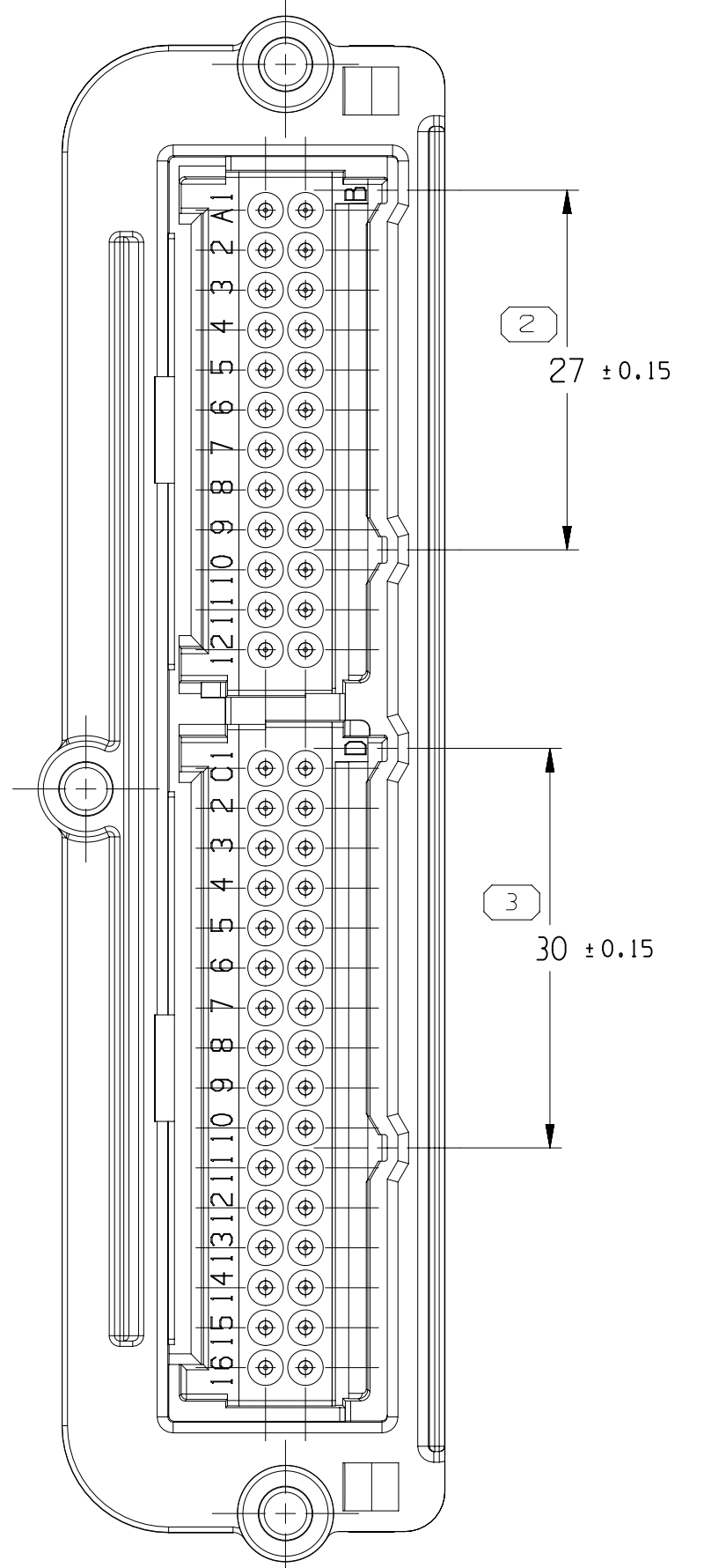
TYPE 103 SAME AS TYPE 101 EXCEPT AS SHOWN SCALE 2:1
