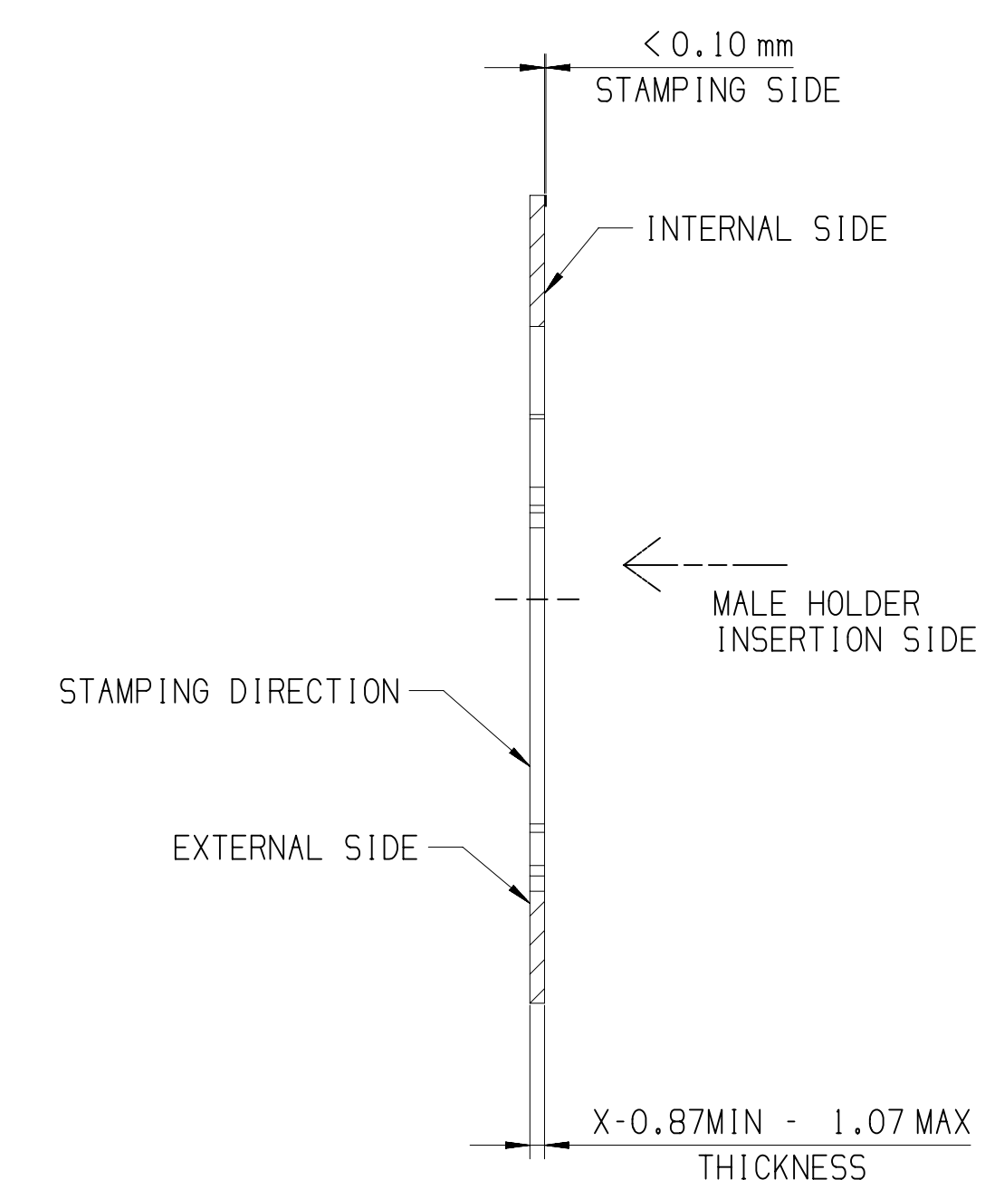
SECTION H-H
