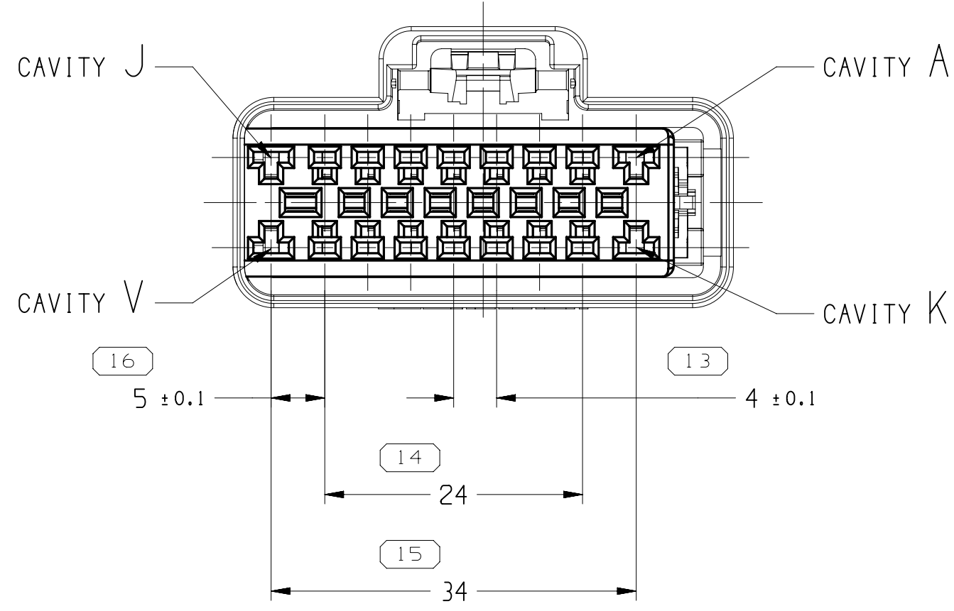
TYPE 105 SAME AS TYPE 101 EXCEPT AS SHOWN SCALE 2:1
