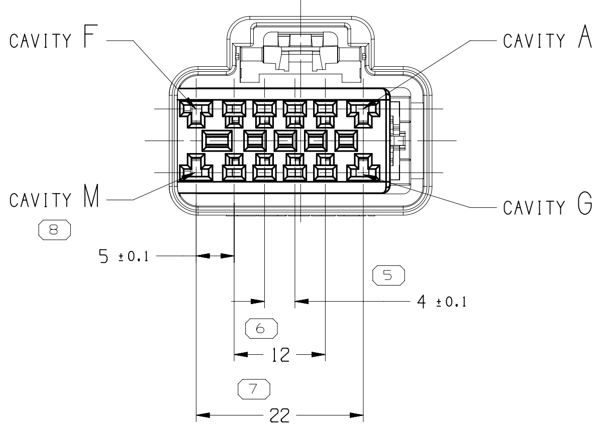
TYPE 102 SAME AS TYPE 101 EXCEPT AS SHOWN SCALE 2:1
