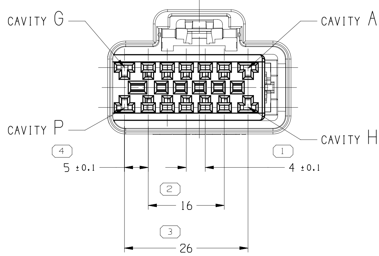
TYPE 103 SAME AS TYPE 101 EXCEPT AS SHOWN SCALE 2:1
