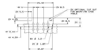
MATING CIRCUIT BOARD INFORMATION SCALE 1:1
