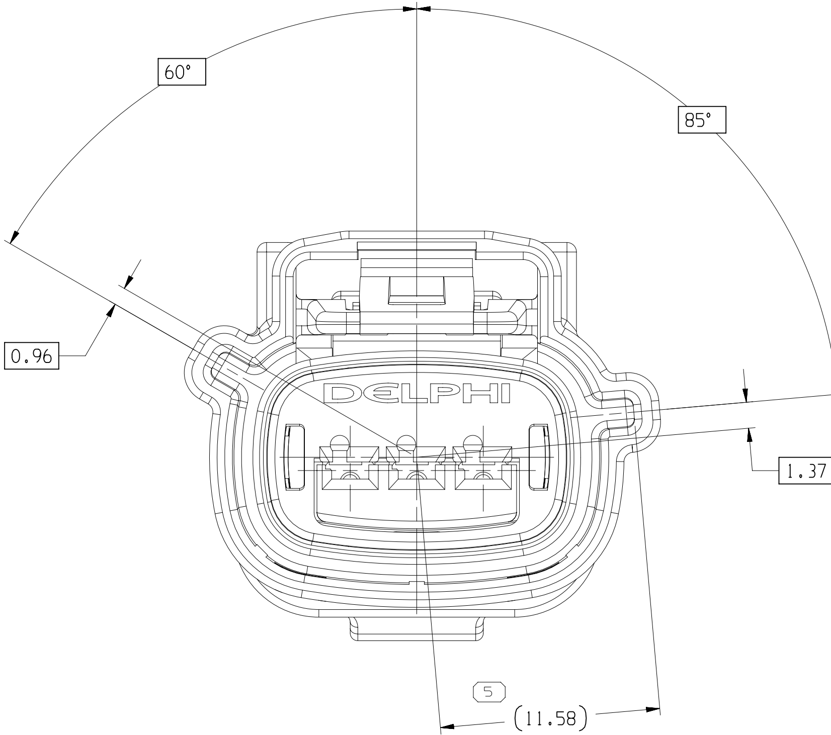
TYPE 106 SAME AS TYPE 101 EXCEPT AS SHOWN
