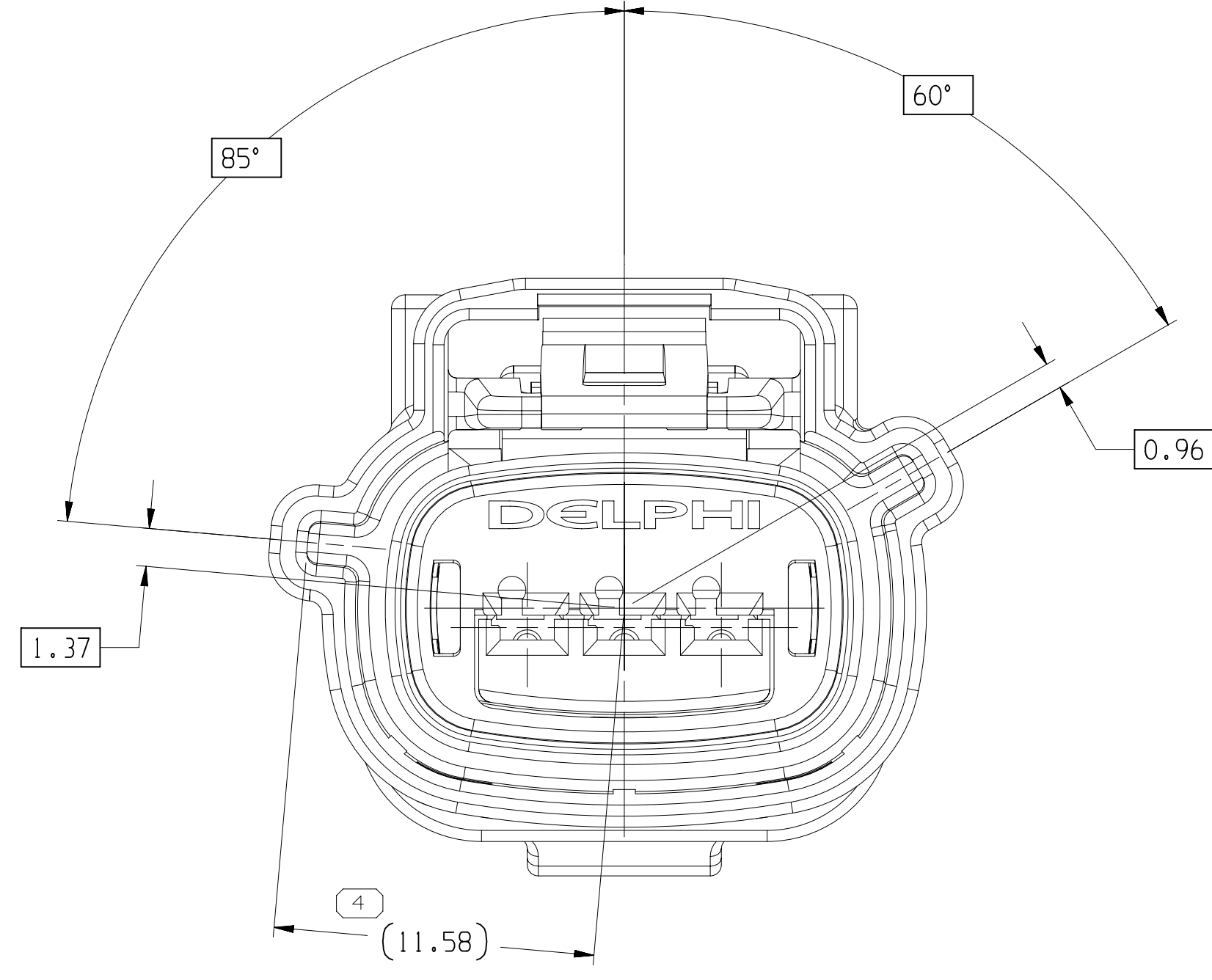
TYPE 105 SAME AS TYPE 101 EXCEPT AS SHOWN
