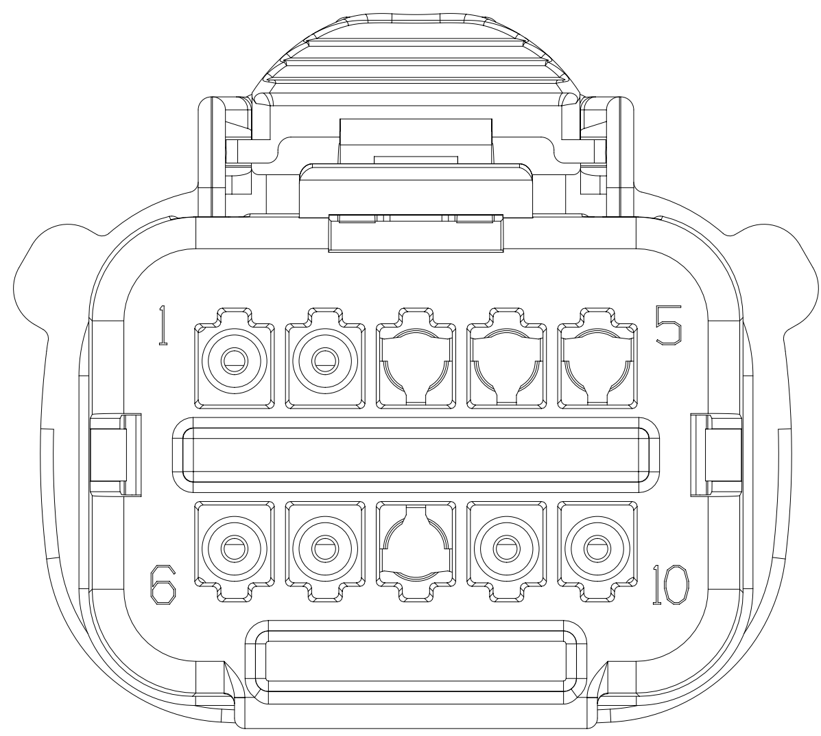
TYPE 202 SAME AS TYPE 201 EXCEPT AS SHOWN
