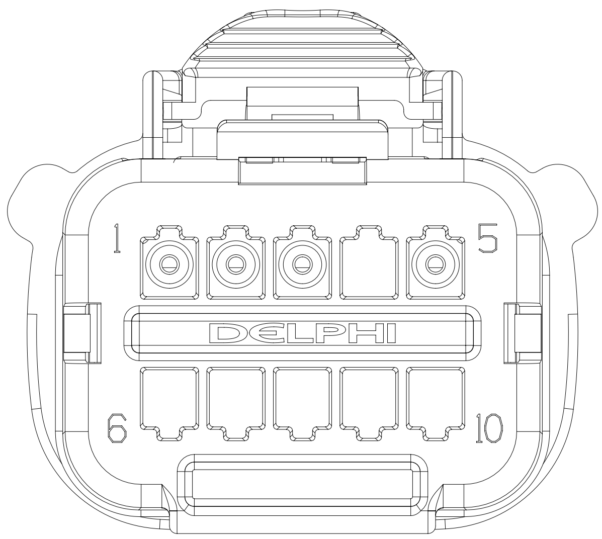
TYPE 206 SAME AS TYPE 201 EXCEPT AS SHOWN
