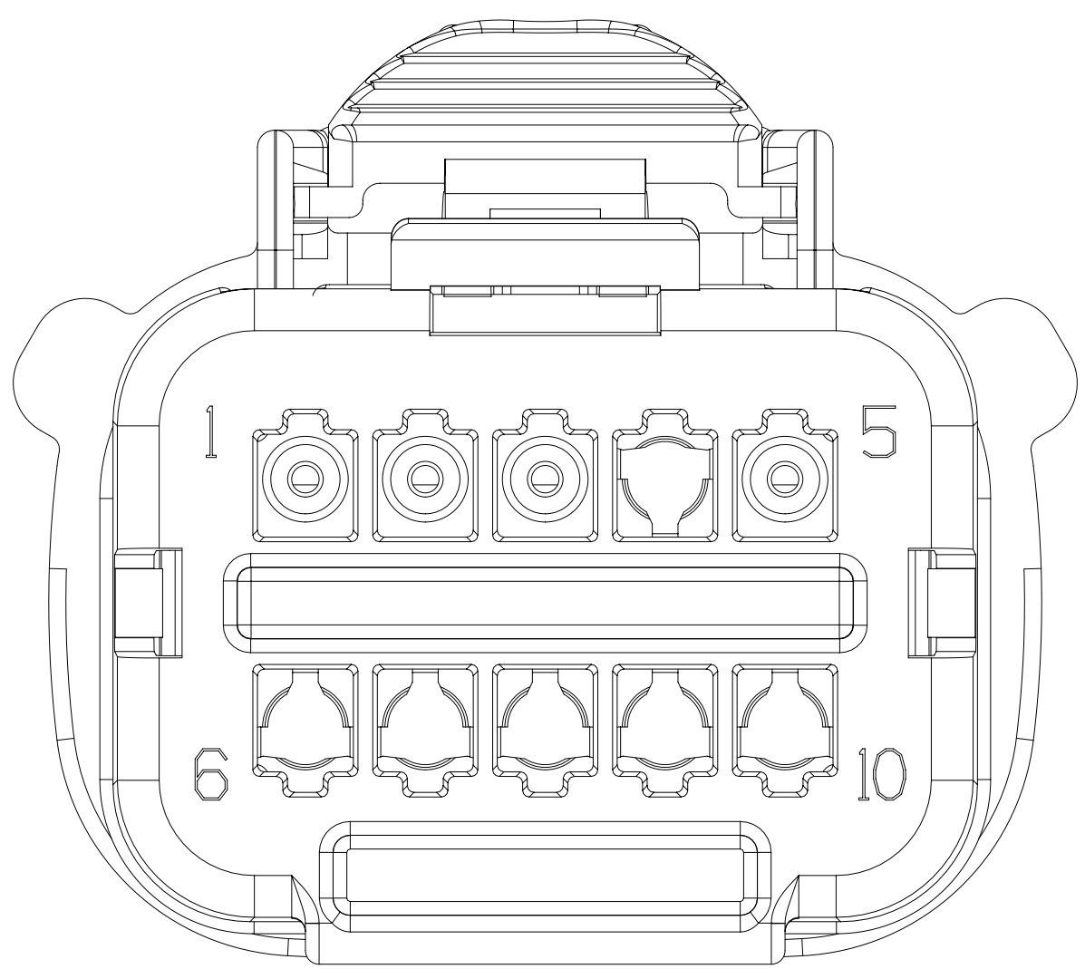
TYPE 207 SAME AS TYPE 201 EXCEPT AS SHOWN
