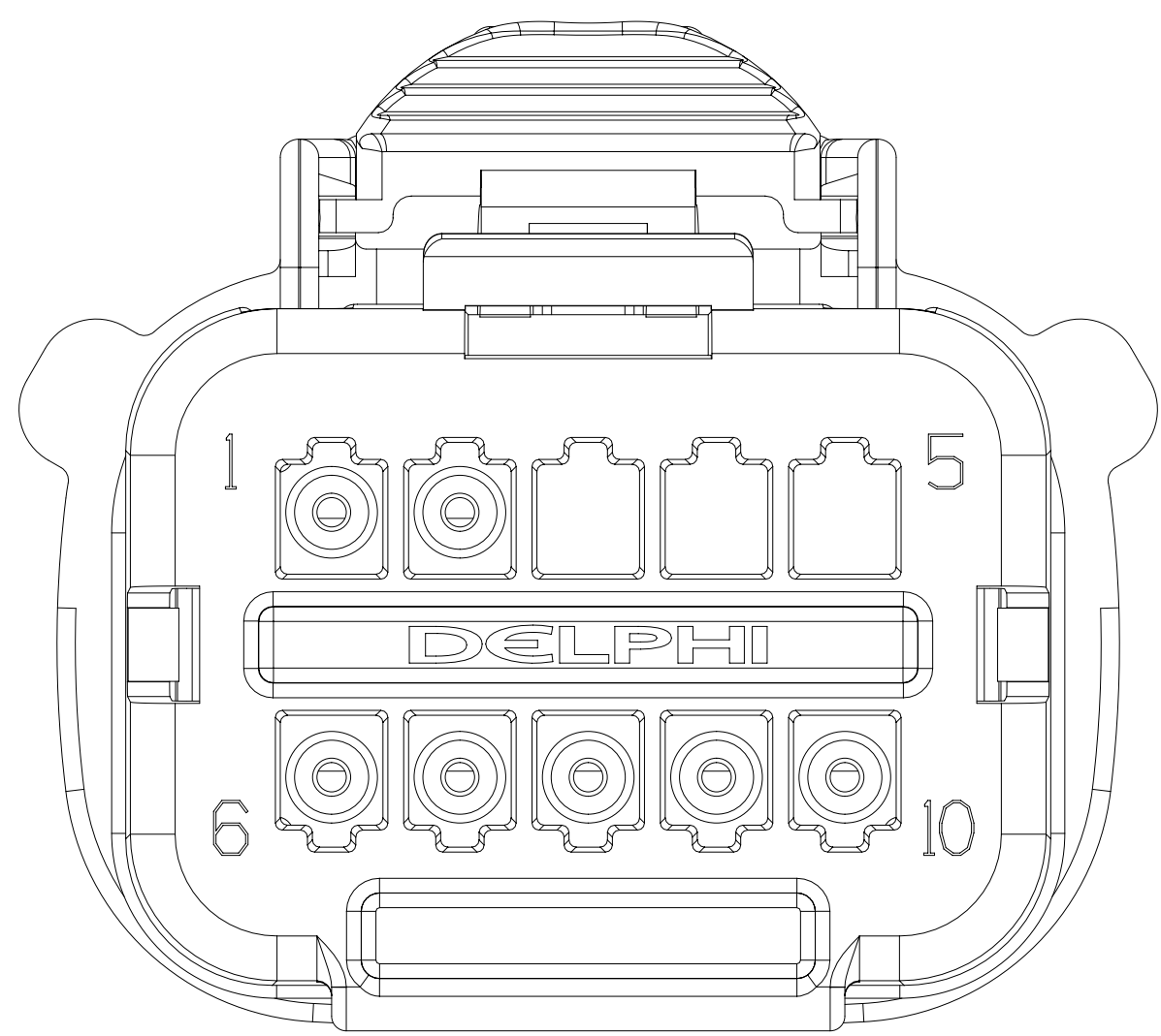
TYPE 203 SAME AS TYPE 201 EXCEPT AS SHOWN
