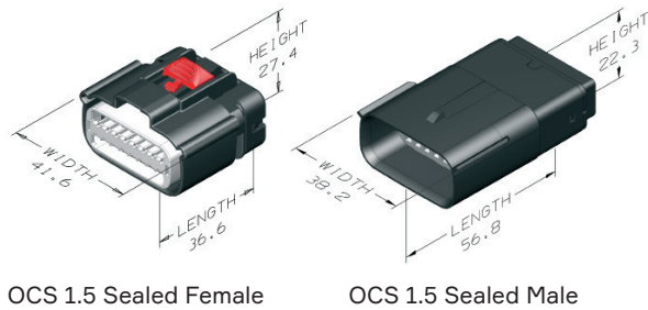
OCS 1.5 Sealed Female
