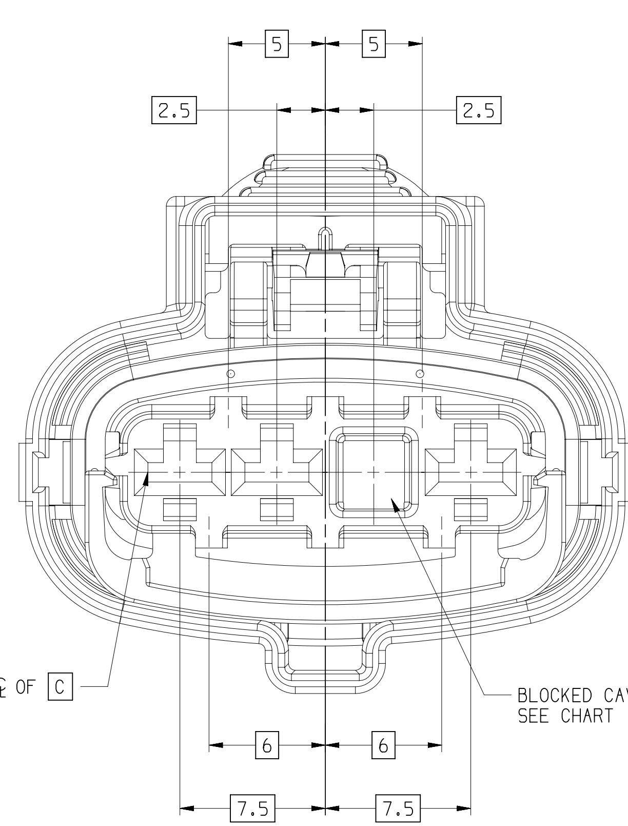
TYPE 205 SAME AS TYPE 201 EXCEPT AS SHOWN
