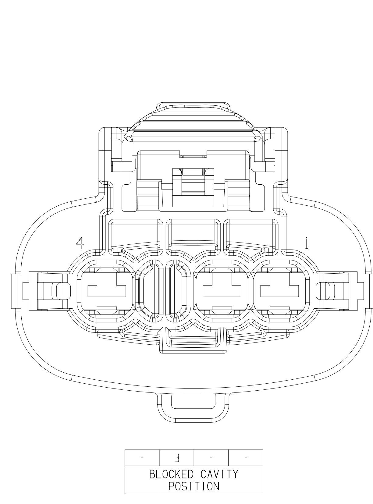
BLOCK CAVITY LAYOUT CONFIGURATION TYPE VIEW / VISUAL AID
