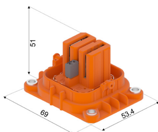
Header type 2
