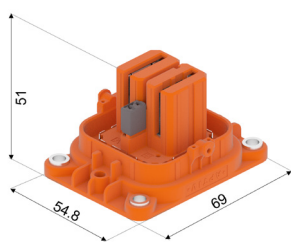
Header type 1
