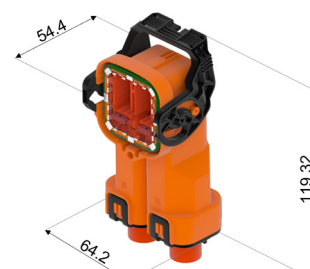
Mating Connector 90°
