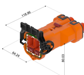
Mating Connector 180°
