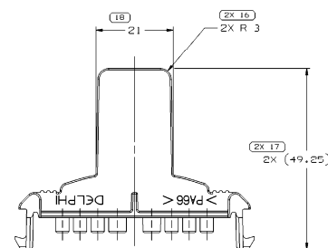
TYPE 102 SAME AS TYPE 101 EXCEPT AS SHOWN
