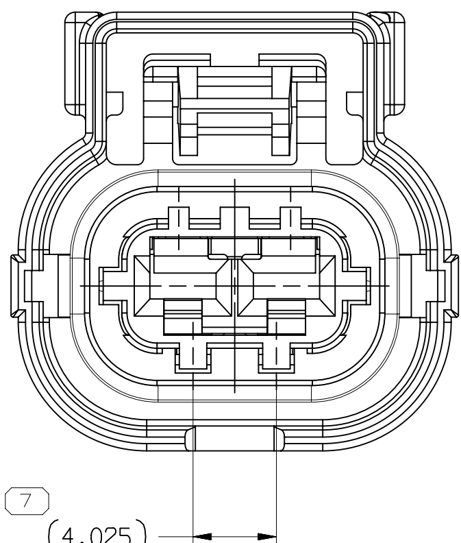
TYPE 105 SAME AS TYPE 102 EXCEPT AS SHOWN THIS CONNECTOR IS A NON-STANDARD VARIANT OF KEY B AND IS INTENDED FOR USE ONLY WITH ONE SPECIFIC NON-STANDARD INTERFACE AND SHOULD NOT BE USED IN ANY OTHER APPLICATION
