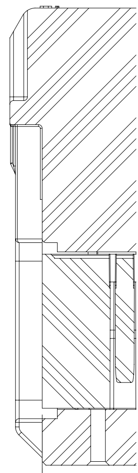
SECTION B-B
