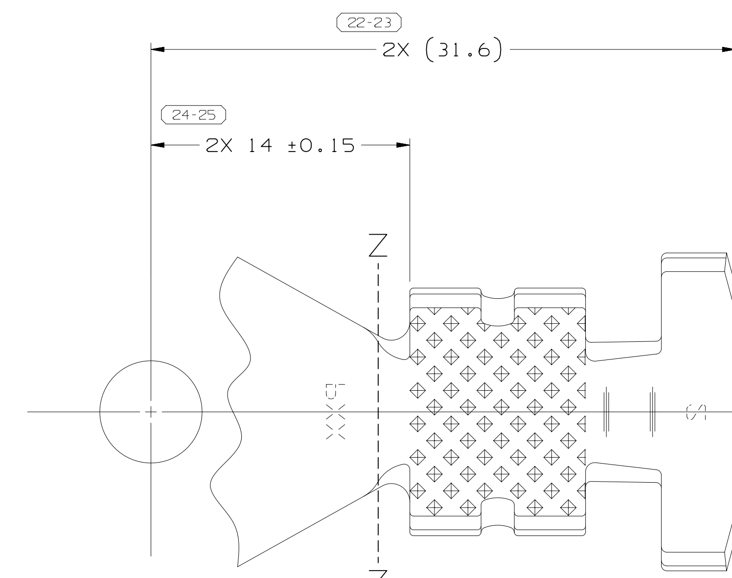
( 32 MM 2 ) TYPE 821/822 SAME AS TYPE 801/802 EXCEPT AS SHOWN
