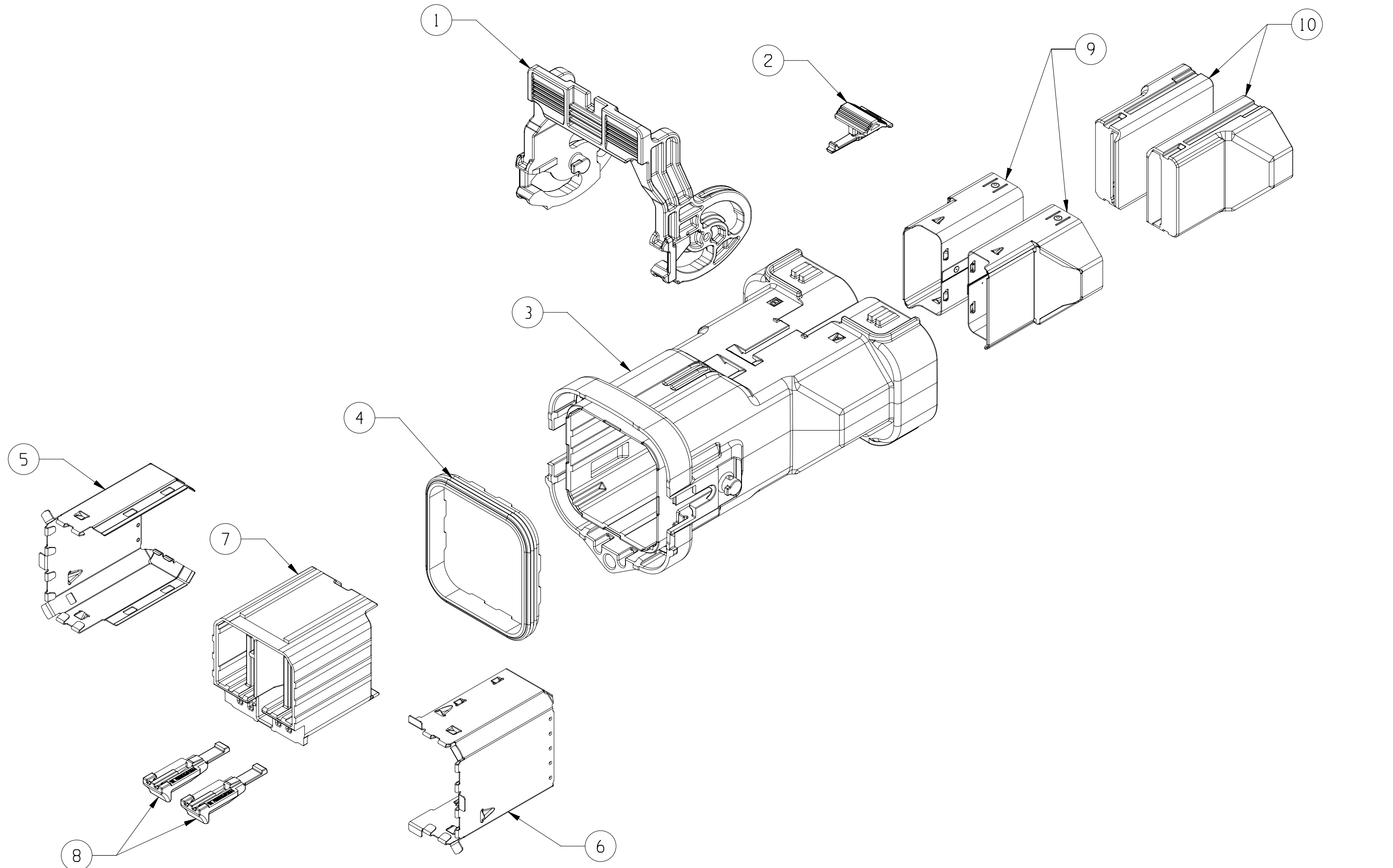
EXPLODED VIEW SCALE 1:1
