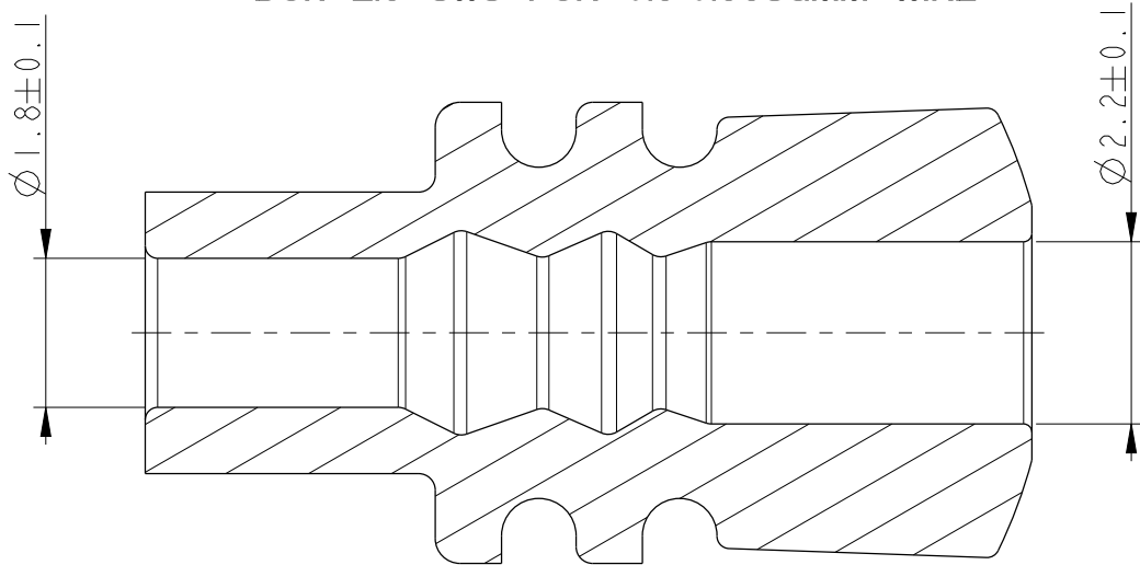
F610400 DCK 2.8 SWS FOR 1.25SQMM WIRE
