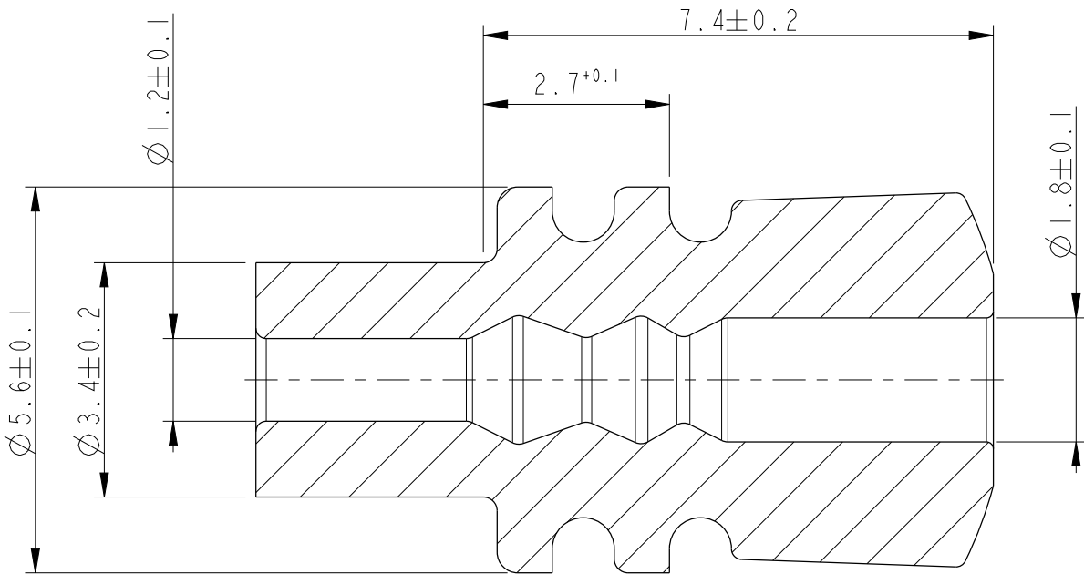
F510400 DCK 2.8 SWS FOR 0.5-0.85SQMM WIRE
