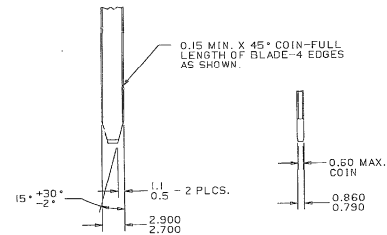
BLADE DETAIL SCALE 4:1
