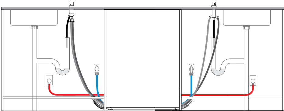
SINGLE AIR GAP INSTALLATION
