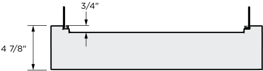
RECESSED PRE-FINISHED TOE KICK 1 9/16" - 3 15/16" DEPTH
