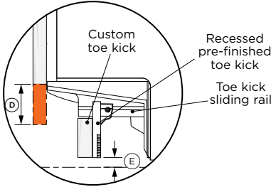
SECTION DETAIL VIEW 1 TOE KICK DEPTHS 2 3/26" - 4 3/4"
