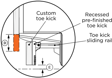
SECTION DETAIL VIEW 1 TOE KICK DEPTHS 1 9/16" - 4 3/4"
