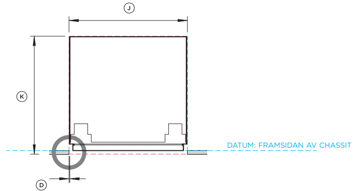
PLANVY
