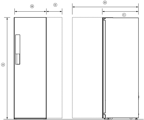
ISOMETRIC VIEW
