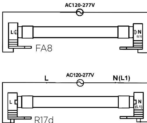
WIRING DIAGRAM
