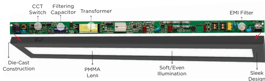
LINEAR DRIVER HOUSED IN FRAME
