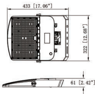
65/873 Yoke Mount
