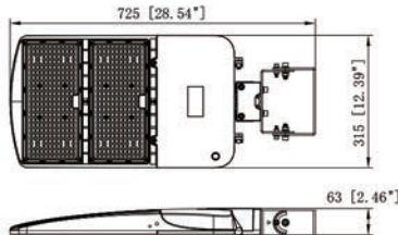
65-872 Trunnion Mount
