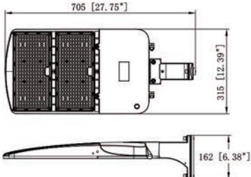
65-871 Direct Mount
