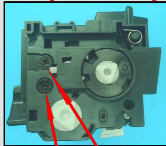
Right side of cartridge.
