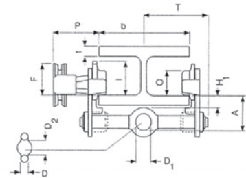
Malli HTP 500 - 5000 kg
