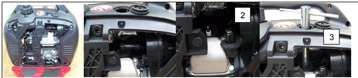
Figure 12: Spark plug
