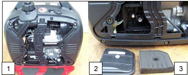
Figure 11: Air filter
