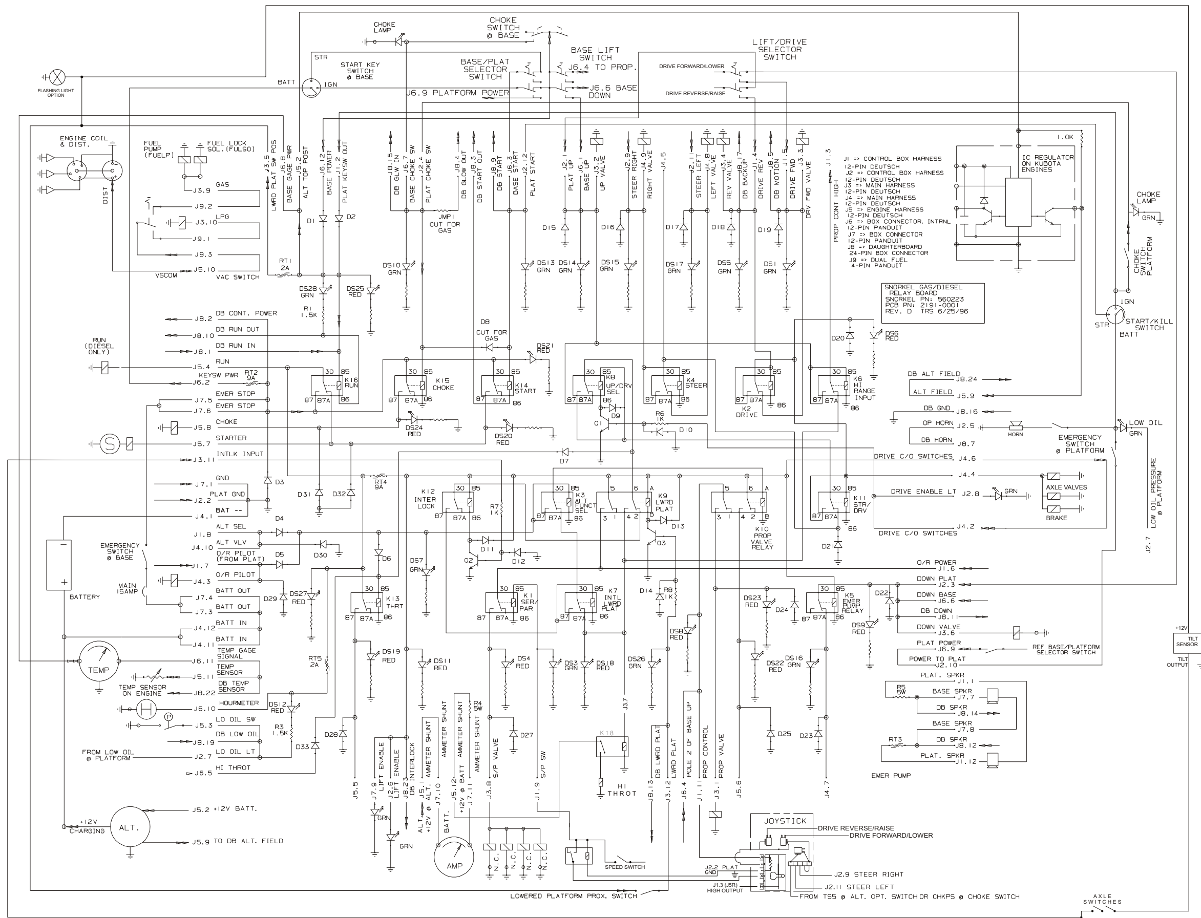
TITLE Electrical Schematic, Standard, Snorkel Models SR3370 & SR2770, V2 Machines without Stabilisers
