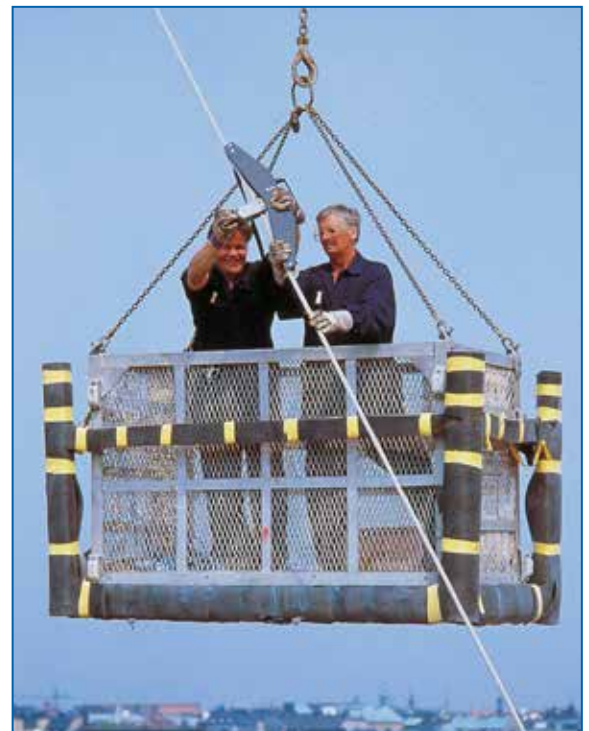
Also when stay ropes are difficult to reach the lightweight RTM 20D is easy to handle. The picture shows control of tension from a crane operated working platform.
