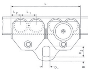
Malli HTG 20000 kg
