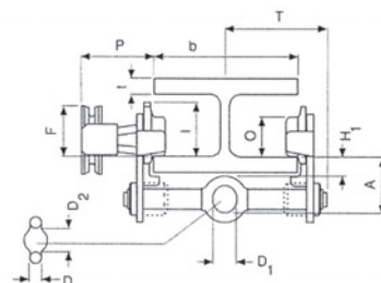
Malli HTP 500 - 5000 kg
