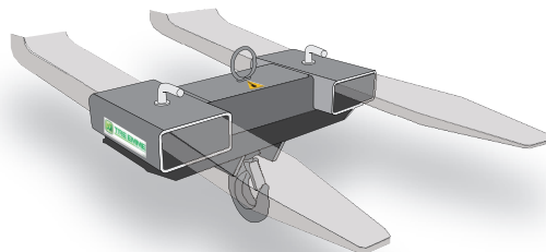
Fork-mounted hook
