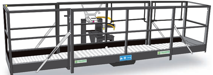
Extendible slewing platform
