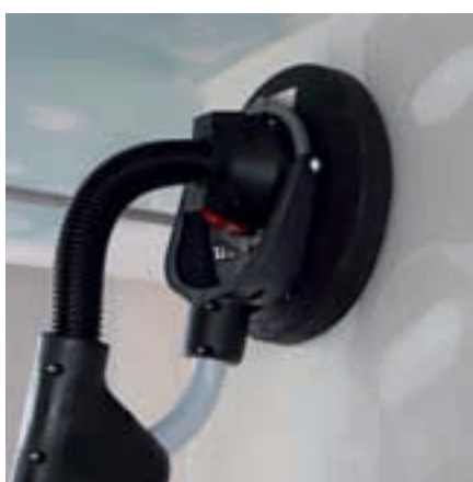
The universal-joint mounting of the sander head allows it to adapt to any inclination and angle.
