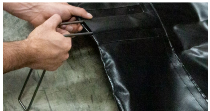
Slip angle L-brackets into protective pockets to keep walls upright, no sagging.
